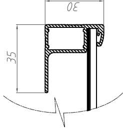
Frame Cross Section A-A
