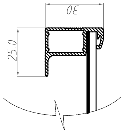
Frame Cross Section B-B
